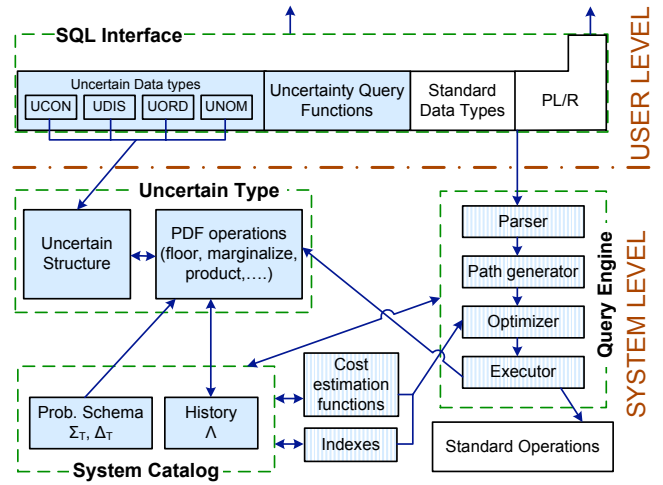
Figure 1: Orion 2.0 Architecture
